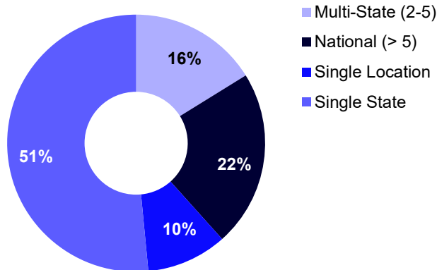
Geographical Spread
